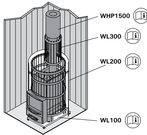
Figure 10. Legend Protection Supplies (all dimensions in millimeters) Abbildung 10. Legend Schutzvorrichtungen (alle Abmessungen in Millimetern)
