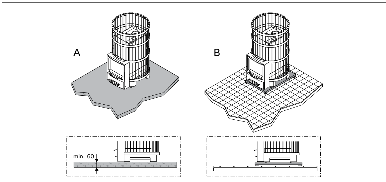
Figure 8. Protecting the floor (all dimensions in millimeters) Abbildung 8. Bodenschutz (alle Abmessungen in Millimetern)
