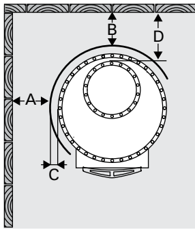
Figure 10. Legend Protection Supplies (all dimensions in millimeters) Abbildung 10. Legend Schutzvorrichtungen (alle Abmessungen in Millimetern)
